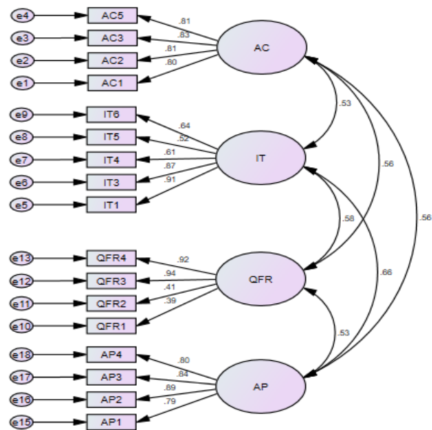
Figure 2: Measurement Model Assessment.
